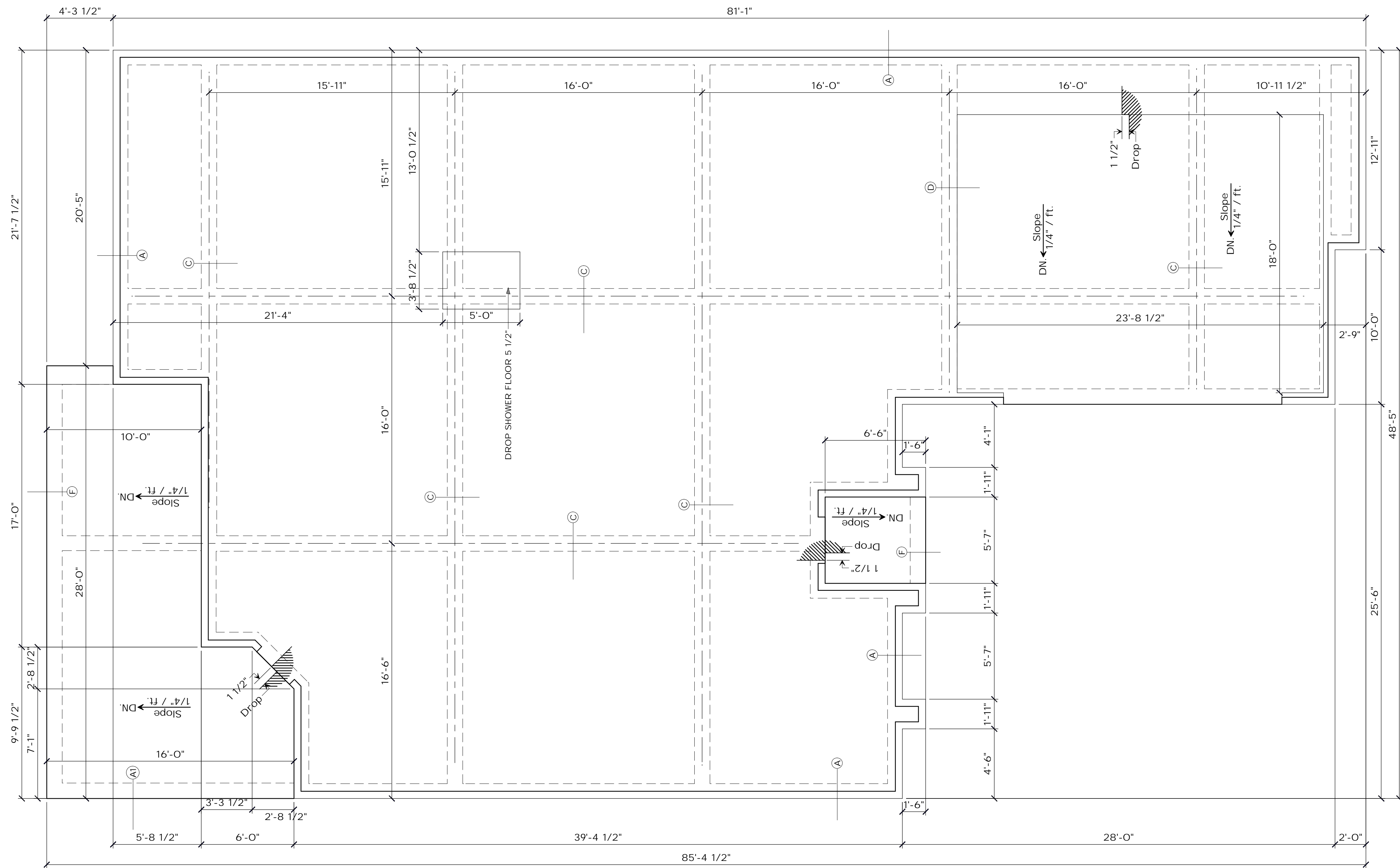
B FOUNDATION PLAN SCALE: 1/4"=1'-0"
